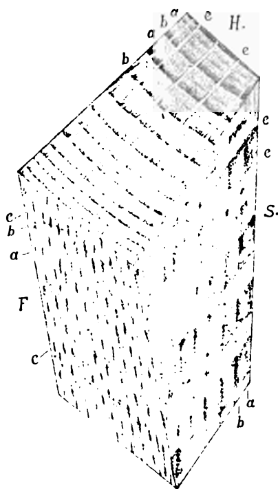
Fig. 10.—Type of Beechwood ( Fagus ).
